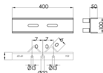
TRAVERSE 400MM
