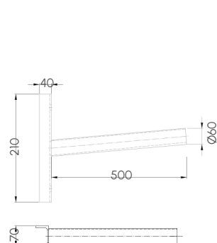
CROSSE MURALE
