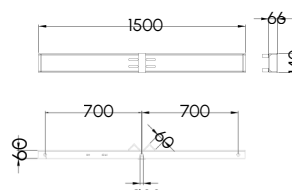
TRAVERSE 1500MM
