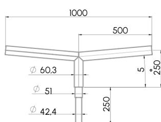
CROSSE DOUBLE
