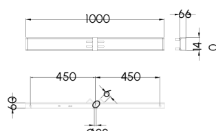
TRAVERSE 1000MM
